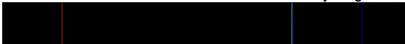
Hydrogen
