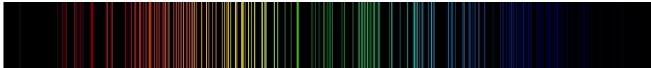
Neon
