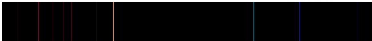
Lithium
